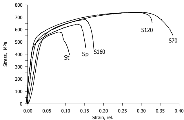
Fig. 6. Slow strain rate test results for samples with various surface layers. Tests performed in MgCl_2 solution at 125°C
