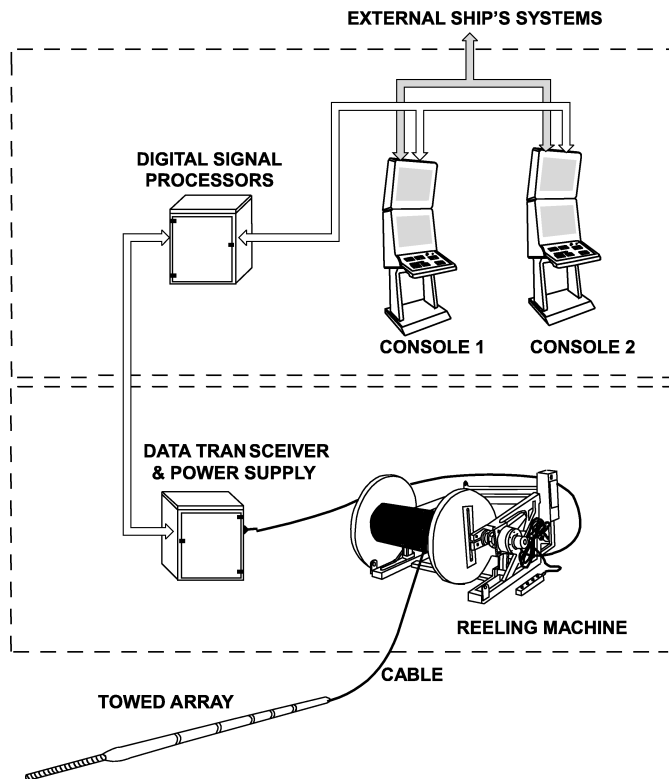
Fig. 2. Sonar structure.
