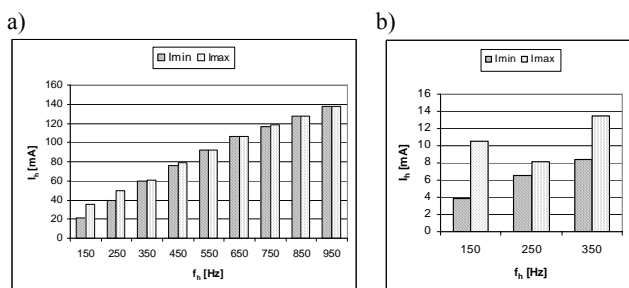
Fig. 8. The effect of harmonic on AC type RCDs tripping current: a) RCD 100 mA, b) RCD 30 mA
