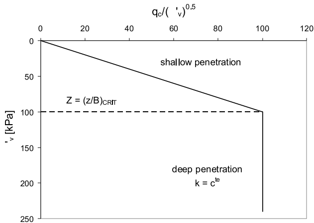
Fig. 4. Idealized penetration resistance scheme
