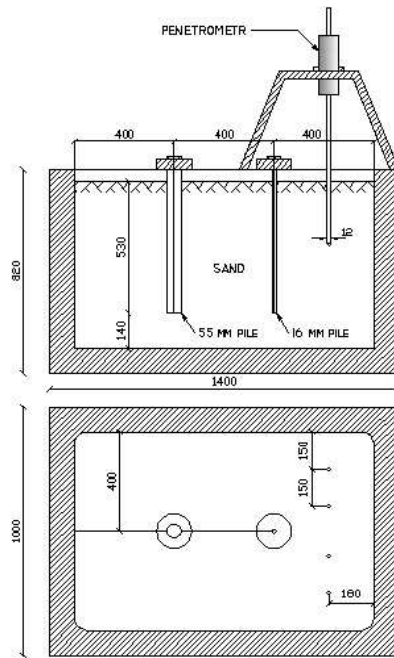
Fig. 11. Container scheme
