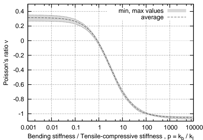
FIG. 4. Influence of the ratio between the bending and longitudinal stiffness p = k_b/k_l on Poisson's ratio \nu during uniaxial compression with smooth edges (using semi-logarithmic scale).
