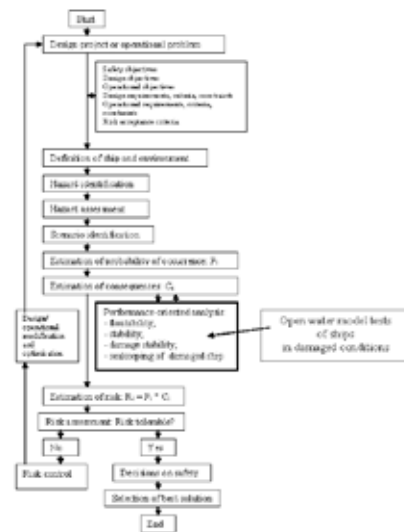
Fig. 2 Logical structure of the risk-based design/operational procedure (method).
