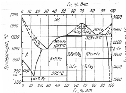
Fig. 1. The equilibrium iron - titanium diagram [5]
