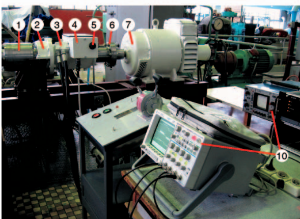
Fig. 3. The laboratory stand for testing the CP propeller servomechanism. Notation: 1 – hydraulic pitch control cylinder placed between flanges of propeller shaft and intermediate shaft; 2 – angular bearing; 3 – hydraulic distributor; 4 – oil timing box with internal control unit; 5 – hand wheel for propeller pitch local setting; 6 – clutch; 7 – shaft driving DC motor; 8 – hydraulic supply unit; 9 – remote control desk; 10 – measurement recording equipment
