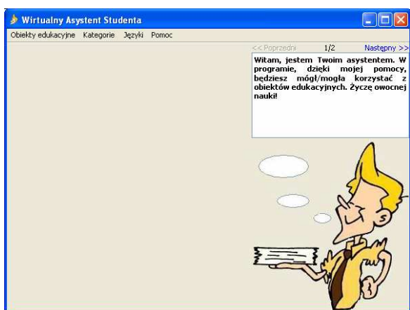
Rys. 2. Agent WAS
