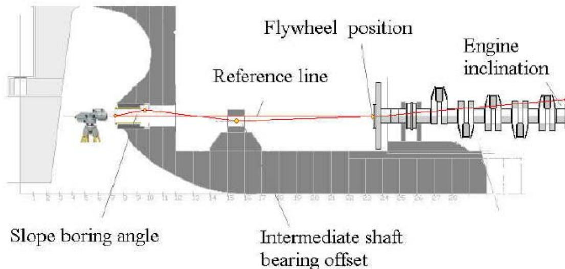
Fig.7. Positioning the Bearings to Actual Design Values [2].
