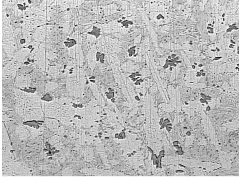
Fig. 2. \kappa -phase precipitates. Unetched specimen. Magn. 500x
