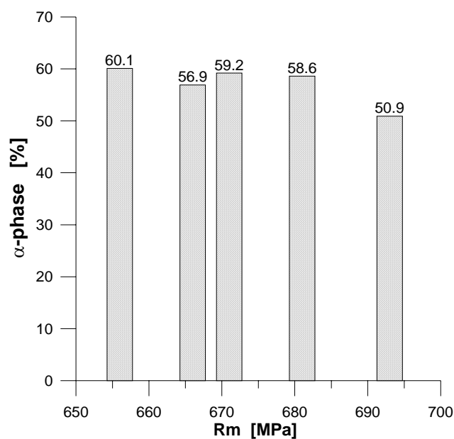
Fig. 3. \alpha -phase contribution in the structure of five casings of BA1055 bronze
