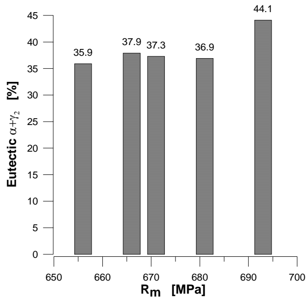
Fig. 4. Eutectoid \alpha+\gamma_2 contribution in the structure of five casings of BA1055 bronze
