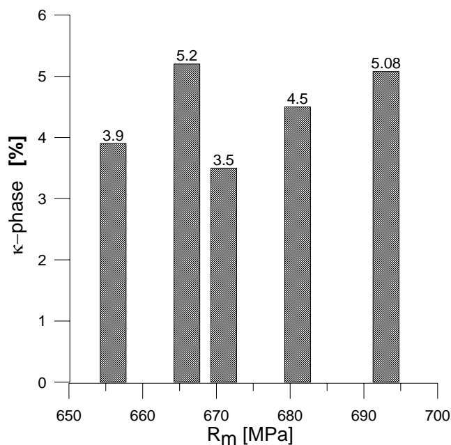
Fig. 5. \kappa phase contribution in the structure of five casings of BA1055 bronze
