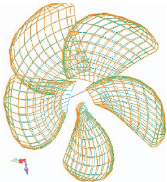
Fig. 10. The designed propeller blades shown in the grid form
