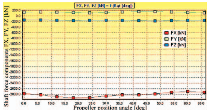
Fig. 14. The components of the unsteady bearing force as the function of propeller angular position
