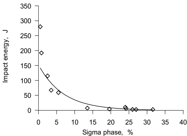
Fig. 18. The influence of \sigma -phase content on impact energy of 2507 superduplex stainless steel
