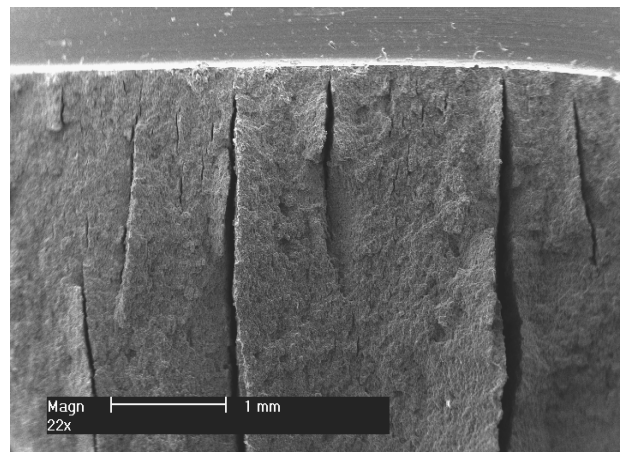
Fig. 13. Fracture surface of specimen treated at 800°C for 1 hour
