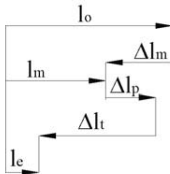
Fig. 12. Dimensional analysis for determining the effective clearance between co-operating elements of hydraulic component in thermal shock conditions
