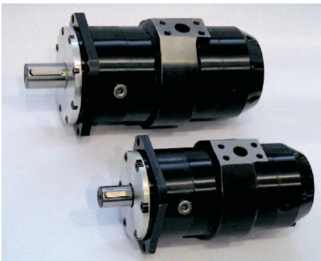
Fig. 2. Camshaft multi-piston pumps PWK-27 and PWK-78 from Hydrotor company [10, 11, 19]
