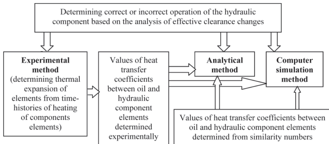
Fig. 5. Methods of determining effective clearance
