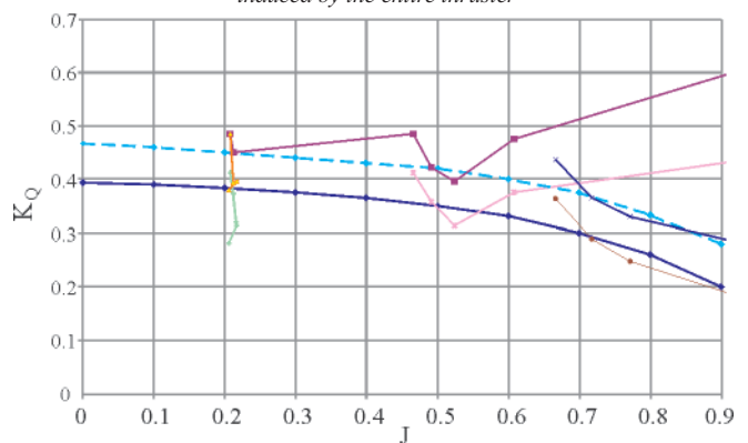
Fig. 2. Results of calculations of torque coefficient K Q
