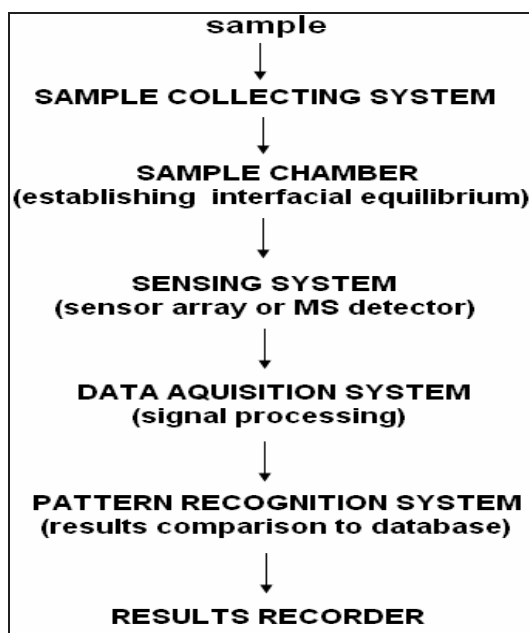
Fig. 3. Electronic nose construction scheme
