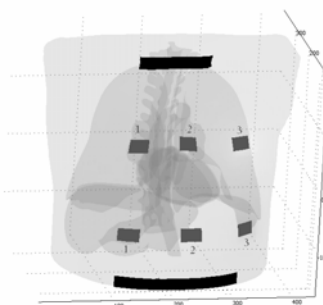
Figure 3. Examined electrode configurations in FEM model.
