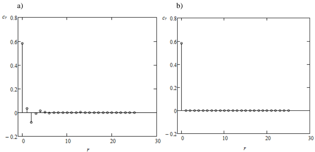
Fig. 8. Device A: a) received values of coefficients c_r ; b) significant values of coefficients c_r .
