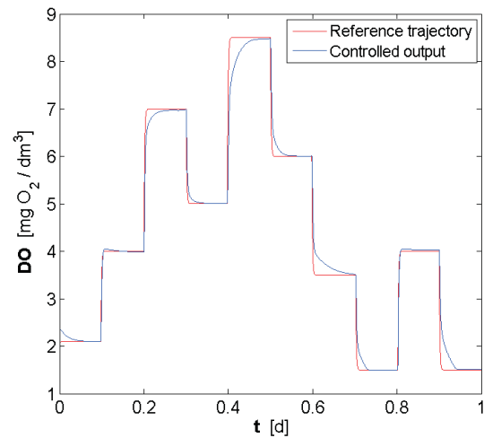
Fig. 16. System performance after calibration.
