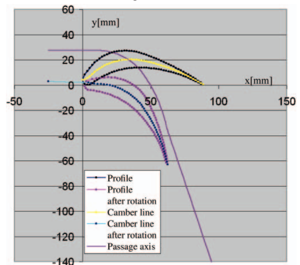
Fig. 4. Profile transformation and creation of the passage axis
