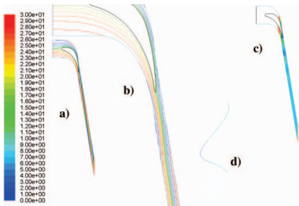
Fig. 8. Results of calculations for profile N3-60, \alpha_u = 36.58^\circ , t/b = 0.6 ; a) streamlines; b) streamlines - enlarged; c) exit angles (scale on the left); d) changes of exit angle \alpha_i along datum +5 mm
