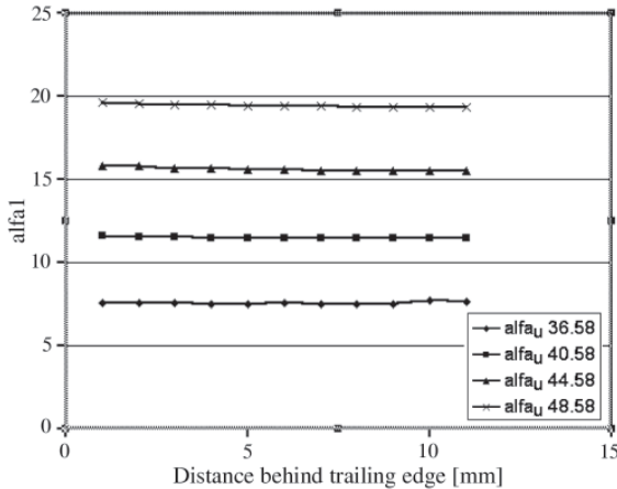
Fig. 7. The angle \alpha_i vs. the distance from the trailing edge
