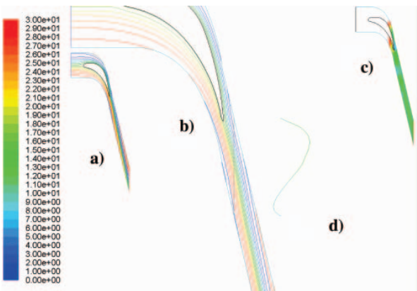
Fig. 9. Results of calculations for profile N3-60, \alpha_u = 40.58^\circ , t/b = 0.6 ; a) streamlines; b) streamlines - enlarged; c) exit angles (scale on the left); d) changes of exit angle \alpha_i along datum +5 mm
