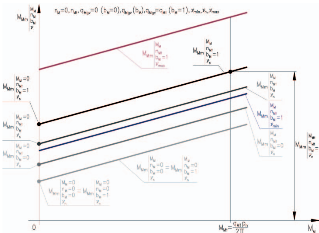
Fig. 6. Torque M_{Mm|M_M, n_M=0, b_M} of mechanical losses in the „shaft – working chambers” assembly of a rotational hydraulic motor with variable capacity q_{Mgv} = b_M q_{Mt} per one shaft revolution as a function of the motor shaft torque M_M – graphical interpretation of the theoretical model (14); motor shaft speeds: theoretical speed n_M, n_M = 0 ; capacity q_{Mgv} per one shaft revolution (coefficient b_M of the change of capacity per one shaft revolution): q_{Mgv} = 0 ( b_M = 0 ), q_{Mgv} = (b_M) q_{Mt} , q_{Mgv} = q_{Mt} ( b_M = 1 ). The impact of working fluid viscosity \nu on friction forces between the „shaft – working chambers” assembly elements and the working fluid occurs mainly in the piston hydraulic motors with casing filled with the working fluid
