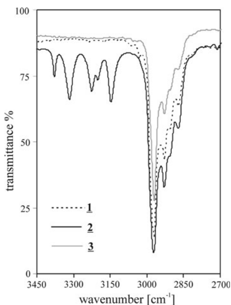
Fig. 5 Solid-state FT-IR spectra of complexes 1–3 in the range 3,400–3,100 \text{cm}^{-1}
