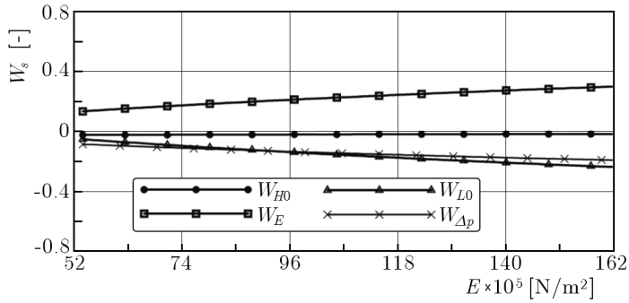
Fig. 9. Relative sensitivity coefficients calculated for M3 model vs. Young's modulus E
