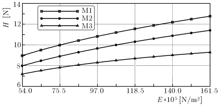
Fig. 5. Junction force H in M1, M2, M3 models vs. Young's modulus E
