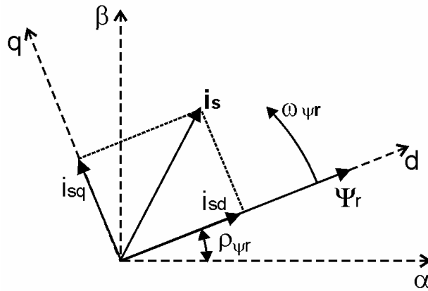
Figure 7. Field oriented control in coordinate system dq connected with rotor flux \psi_r
