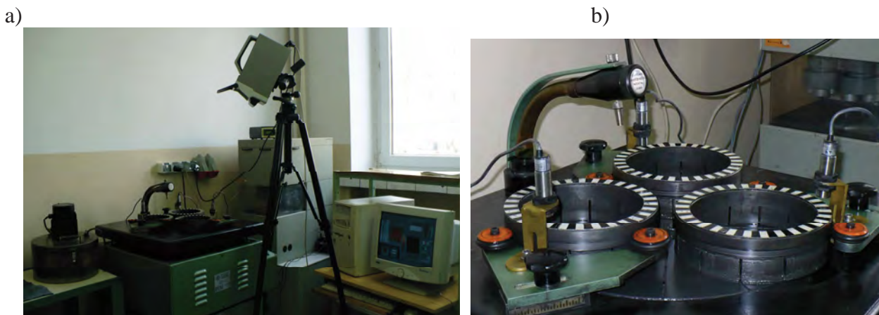
Fig. 1. Experimental setup; a) general view, b) executory system
