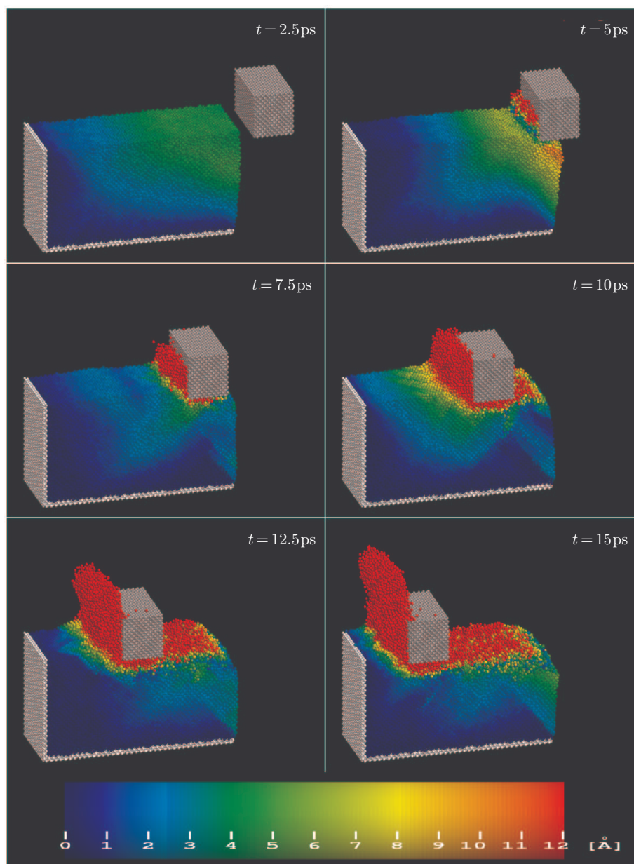
Figure 30. Atomic configurations at selected instants for the initial system temperature of T = 300\text{K} . Machining depth 2a , machining speed v = 1000\text{m/s}
