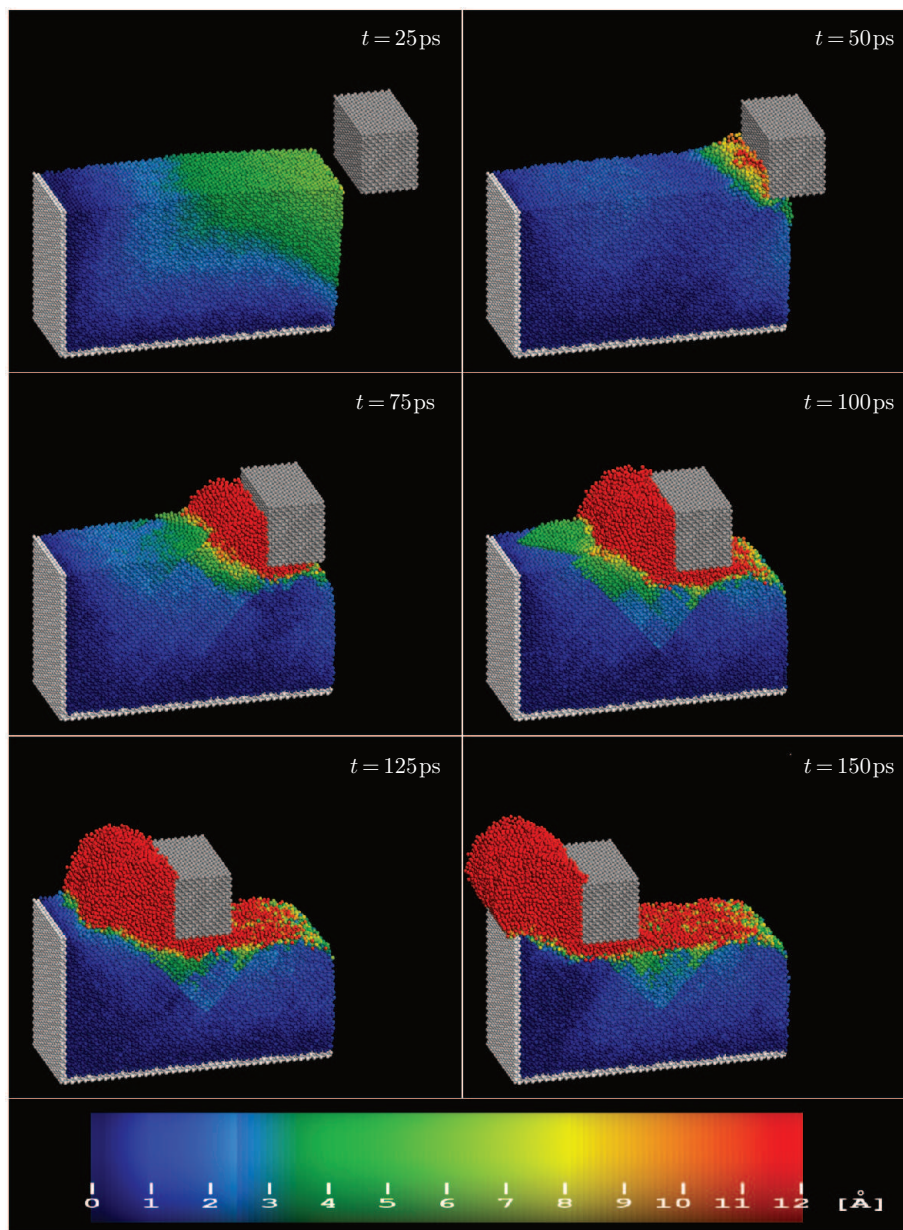
Figure 11. Atomic configurations at selected instants for the initial system temperature of T = 500 K. Machining depth 2a , machining speed v = 100 m/s
