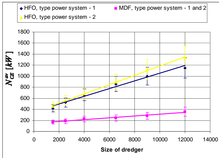
Fig.1. Thermal power demand taking place on six analyzed suction hopper dredgers
