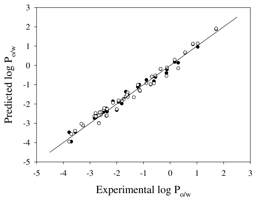
Figure 2. The relationship of experimental and predicted \log P_{O/W} values determined using measured ( \bullet ) and calculated LFER parameters ( \circ ).
