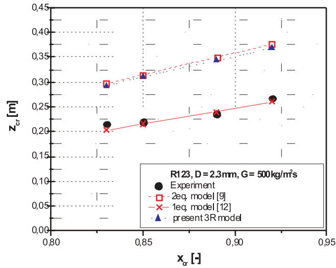
Figure 14. Influence of the R123 mass flux density on the simulation results accuracy for D = 2.3 mm.
