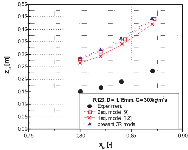
Figure 12. Comparison between the modeling and experimental data for R123 working medium in the channel with D = 1.15 mm and G = 300 kg/m 2 s.
