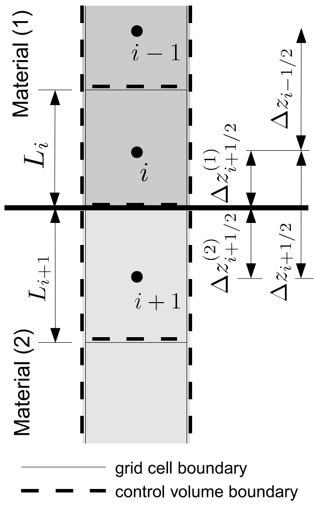
Figure 2: Cell-centered spatial discretization.
