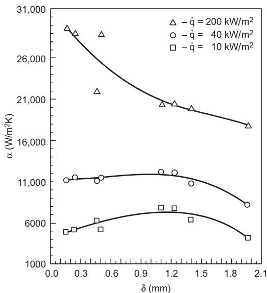
Figure 1 Effect of aluminium coating thickness on heat transfer coefficient ( \varepsilon > 0.50 ).
