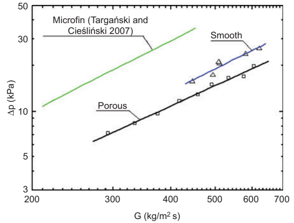
Figure 20 Pressure drop for flow boiling of pure R22 inside a smooth tube and a tube with porous coating.
