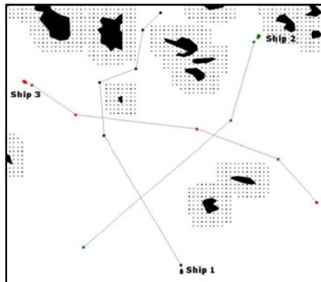
Figure 5. Restricted water basic scenario #1 – simulation starting screenshot (dotted areas depict non-approachable regions)
