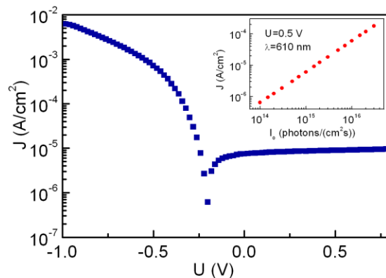
Fig. 1. Current versus voltage at \lambda = 610\text{nm} and I_0 = 10^{15} photons/( \text{cm}^2\text{s} ) and current versus light intensity (inset).
