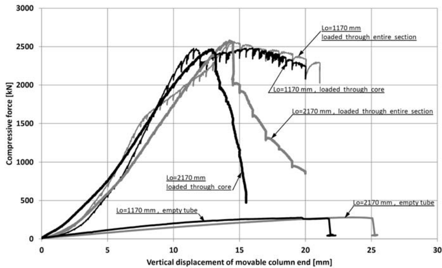
Fig. 5: Load-displacement relations of investigated columns
