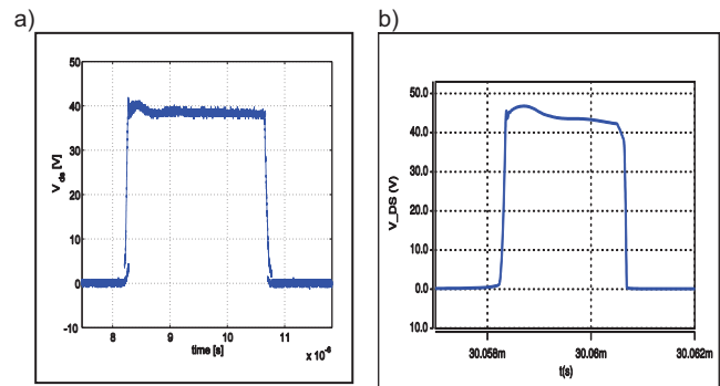
Fig.3. MOSFET voltage waveforms; a) measured b) simulated
