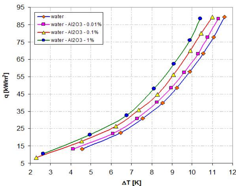
Fig. 3. Influence of concentration of water-Al 2 O 3 nanofluid while boiling at 10 kPa
