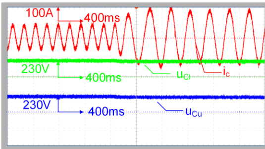
Fig.14. The voltage on upper u_{Cu} and the lower u_{Cl} capacitor of DC-link u_{Cu} , and phase current i_c during load change from 0.05 to 0.45 pu, Fundamental frequency: 5[Hz], DC-link voltage U_{dc}=460V
