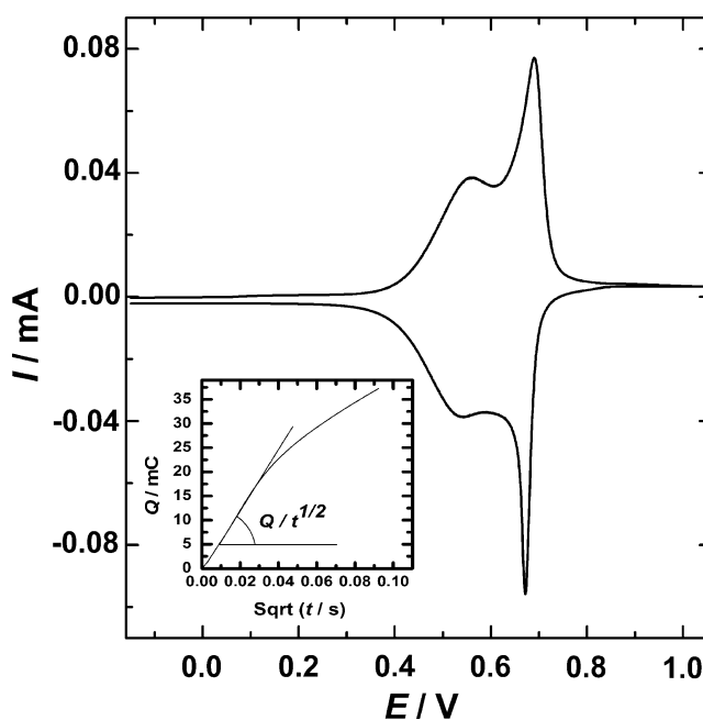
Fig. 2 Cyclic voltammetric response of NiHCF film on glassy carbon electrode recorded in 0.5 \text{mol dm}^{-3} \text{K}_2\text{SO}_4 . Scan rate, 50 \text{mV s}^{-1} . Inset illustrates chronocoulometric response obtained upon application of the anodic potential step from 0 to 0.85 V
