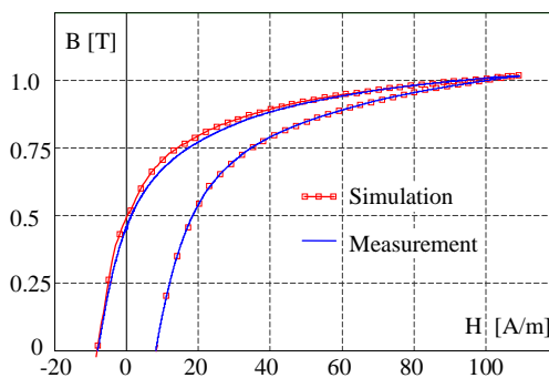
Fig.12. Simulated and measured symmetrical minor hysteresis loops – verification of applied model
