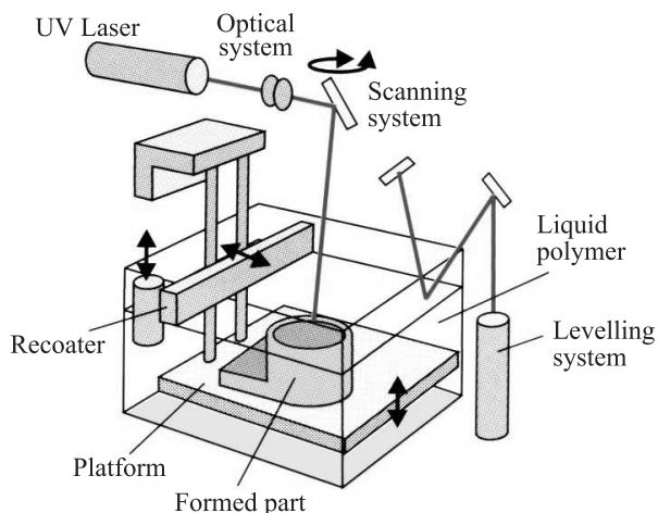
Fig. 1. Schematic illustration of the stereolithography process [9]
