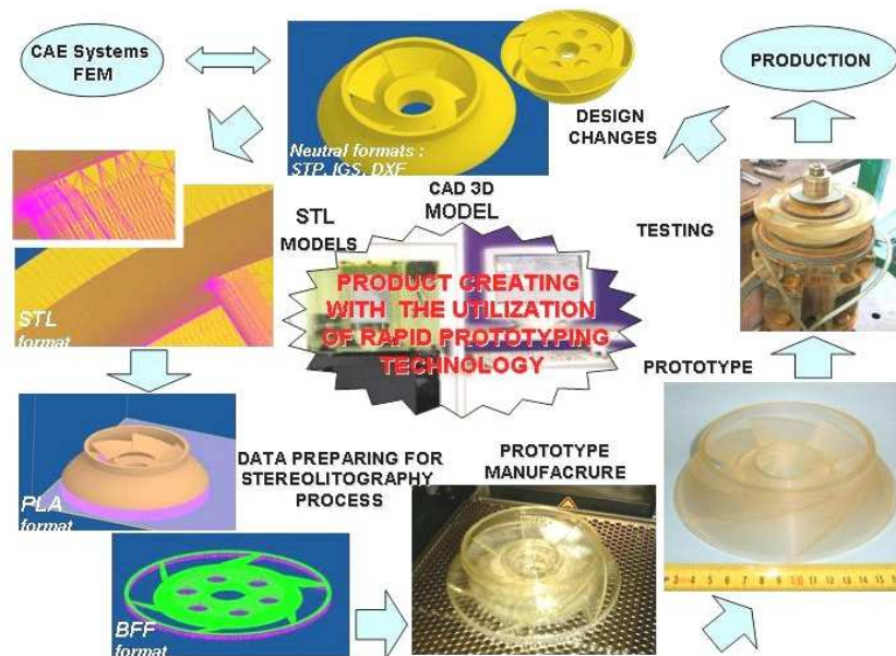
Fig. 3. Cycle of the integrated product development of the pump rotor with the utilization of Stereolithography Technology (SLA)
