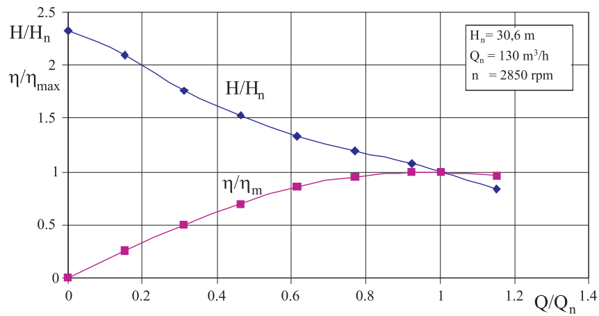
Fig. 5. Dimensionless characteristic of the two stage deep-well pump. The rotor and the diffuser were made using Rapid Prototyping Technology/Stereolithography Process [10]
