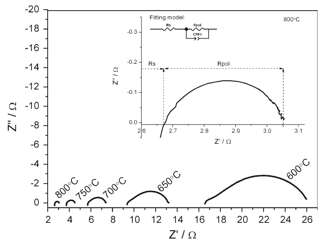
Fig. 3 Typical impedance spectra of STF50/YSZ/STF50 symmetrical electrode measured in the temperature range from 600°C to 800°C
