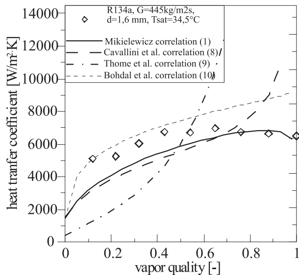
Figure 7. Comparison of heat transfer coefficient for R134a in relation to experimental data due to Bohdal et al. (2011), d = 1.6 mm, G = 445 \text{kg/m}^2\text{s} , T_{\text{sat}} = 34.5 ^{\circ}\text{C} .
