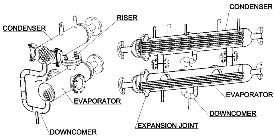
Fig. 2. Axonometric view of the prototype TPTHEx
