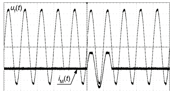
Fig. 5. Oscilloscope of the phase voltage u_f(t) and measurement current i_M(t) of the “Meter-M2”, scale: time 20 ms/div, voltage 100 V/div, current 20 A/div
