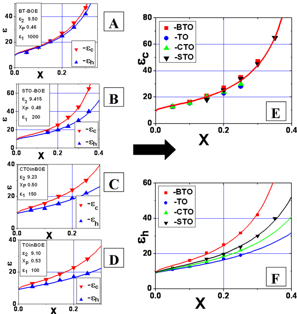
FIG. 5. Dependences of high frequency permittivity \epsilon_h and permittivity calculated from high frequency semicircle \epsilon_c for various powders in BOE. (a) BTO, (b) STO, (c) CTO, (d) TO; (e) \epsilon_c dependence for all powders, (f) \epsilon_h dependence for all powders.
