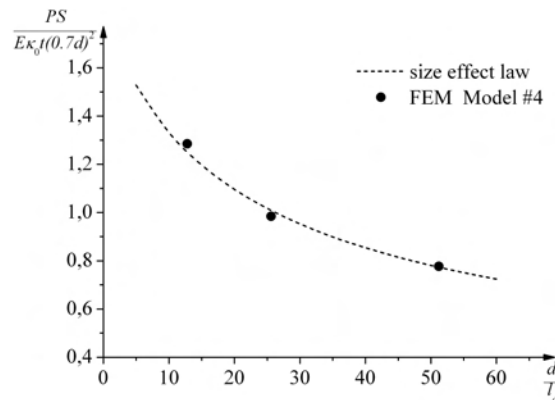
FIG. 8. Calculated deterministic size effect for concrete notched beams subjected to quasi-static cyclic three-point bending (using coupled model ‘4’) as compared with size effect law by BAŽANT [4] ( t – beam thickness, d – beam height, S – beam span).
