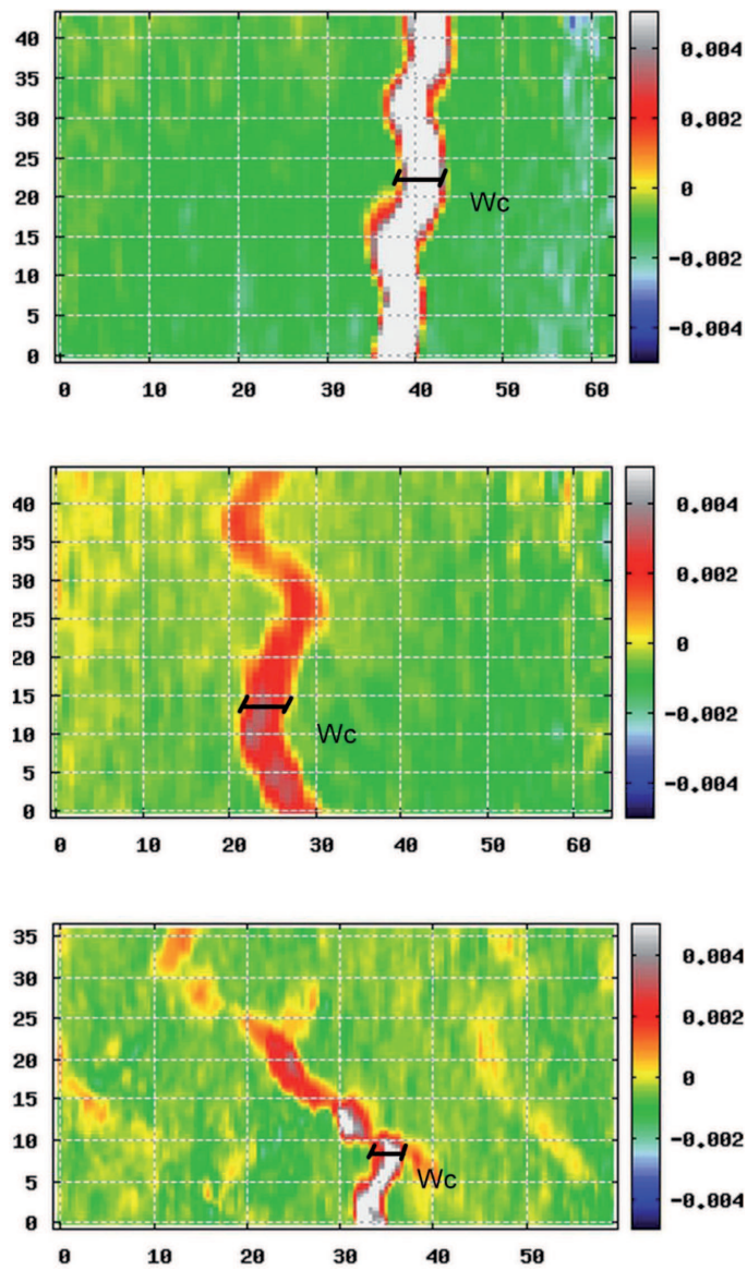
Fig. 4. Formation of localized zone with mean width of w_c = 3.5-4.0 mm directly above notch in 3 different experiments with small-size notched beam 80 \times 320 \times 40 mm 3 using DIC (vertical and horizontal axes denote coordinates in [mm] and colour scales strain intensity) (Skarżyński et al. [14]).
