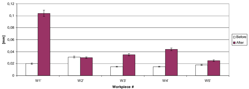
Fig. 9. Plane-parallelism errors recorded after grinding tests T_4 \div T_6
